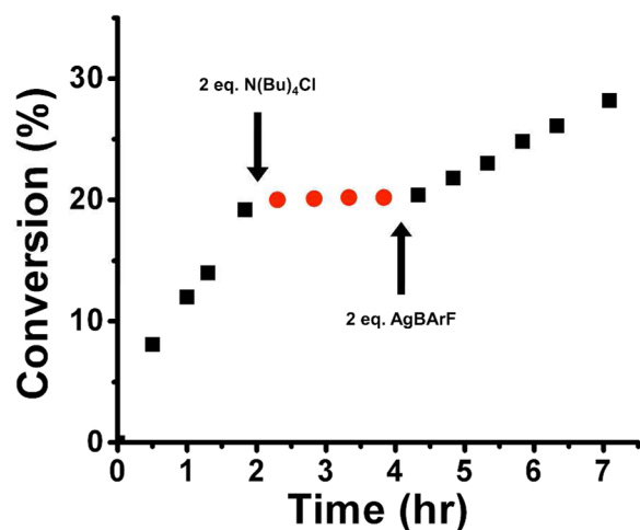
Figure 6. In situ addition of 2 equiv of N(\text{Bu})_4\text{Cl} after 2 h to a solution of fully closed 4 , catalyzing the Friedel–Crafts reaction between indole and nitrostyrene, shows immediate turn-off of catalysis, due to formation of semiopen 3 . In situ re-formation of 4 and re-initiation of activity achieved by the addition of 2 equiv of \text{AgBARF} .
